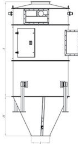
FILTER WITH ROTORFLOW
